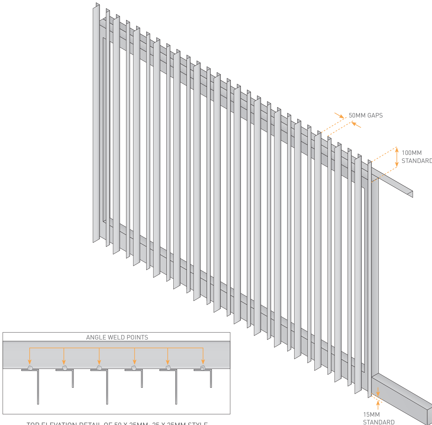
TOP ELEVATION DETAIL OF 50 X 25MM; 25 X 25MM STYLE
