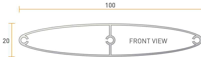
100 x 20 x 1.8mm ELLIPTICAL SLAT with Centre Support Gusset
