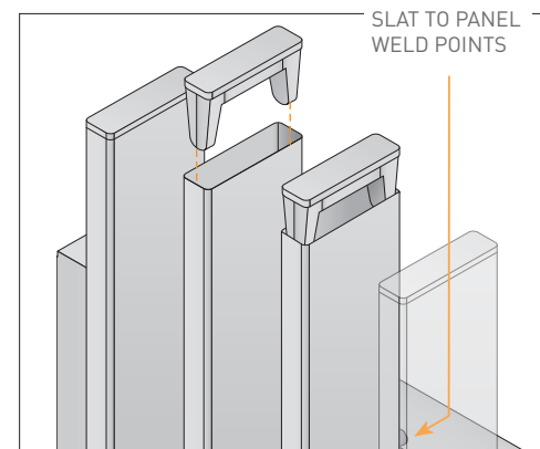
CAST CAP DETAIL
