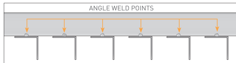
TOP ELEVATION DETAIL OF 40 X 40MM STYLE
