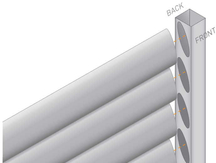
50 X 50MM CNC EXTRUSION DETAIL
