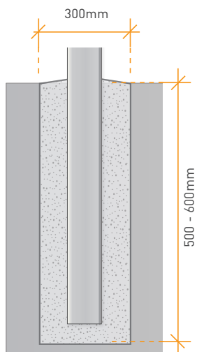
IN GROUND POST DETAIL
