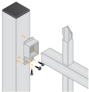
TOP BRACKET
