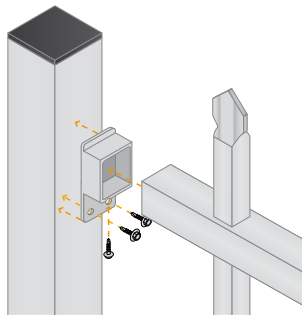
TOP BRACKET
