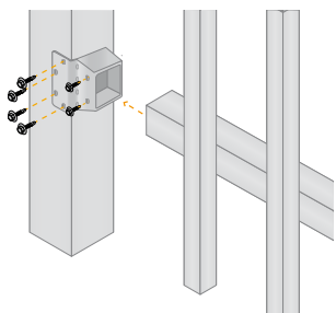
BOTTOM BRACKET
