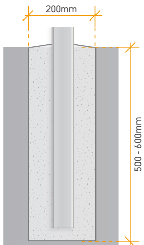
IN GROUND POST DETAIL
