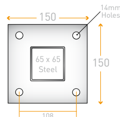
FLANGED (ON SLAB/TIMBER) POST DETAIL
