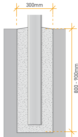
100 x 100 In Ground
