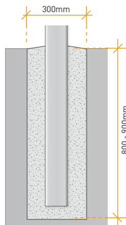
100 x 100 In Ground
