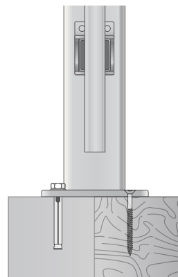
SLAB TIMBER
