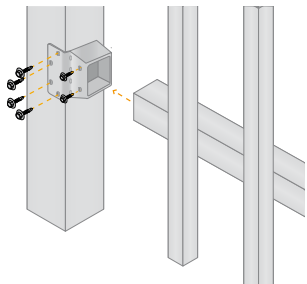
BOTTOM BRACKET
