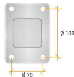
FLANGED (ON SLAB/TIMBER) POST DETAIL
