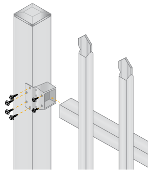
TOP BRACKET
