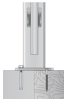
FLANGED (ON SLAB/TIMBER) POST DETAIL
