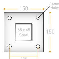
FLANGED (ON SLAB/TIMBER) POST DETAIL
