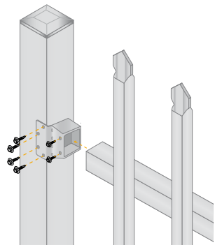
TOP BRACKET
