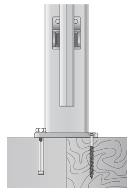
SLAB TIMBER
