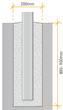
65 x 65 In Ground
