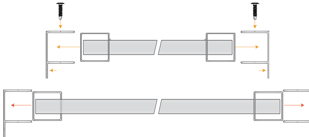
F CHANNEL POST FIXING DETAIL - TOP VIEW
