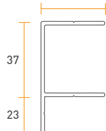
F CHANNEL
