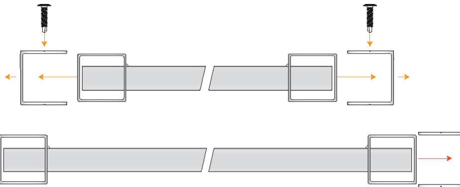
C CHANNEL POST FIXING DETAIL - TOP VIEW
