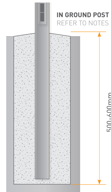
IN GROUND POST END DETAIL
