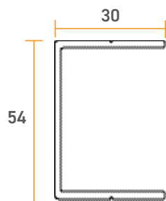
54 x 30mm U CHANNEL
