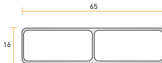
65 x 16 x 1.2mm ELLIPTICAL SLAT with Centre Support Gusset
