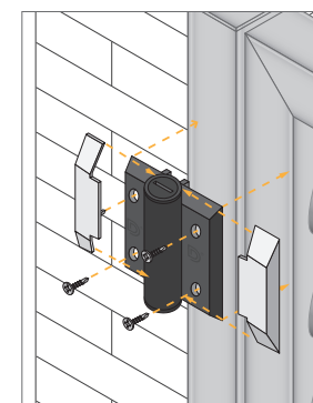
TRU CLOSE REGULAR HINGE
