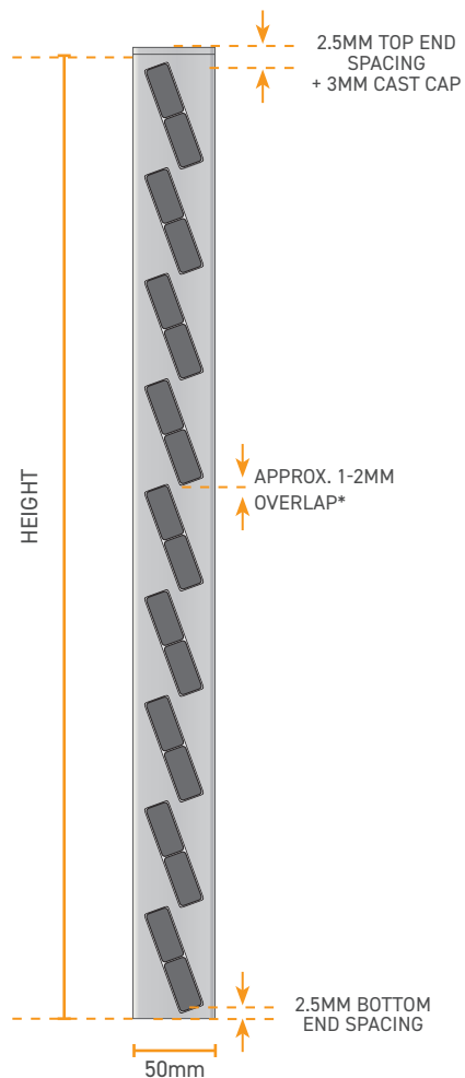
STILE SIDE ELEVATION
