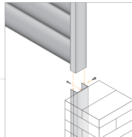
U CHANNEL USED WHEN SLIDING PANEL DOWN FROM TOP
